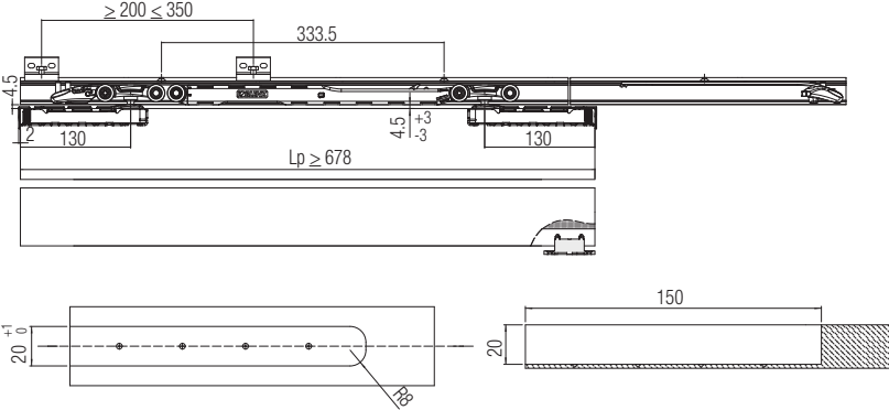
ABS + STOPPER Арт. 0600/80 1ABS
