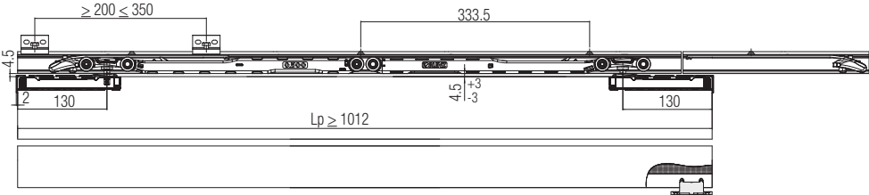
ABS DOUBLE Арт. 0600/80 ABSU
