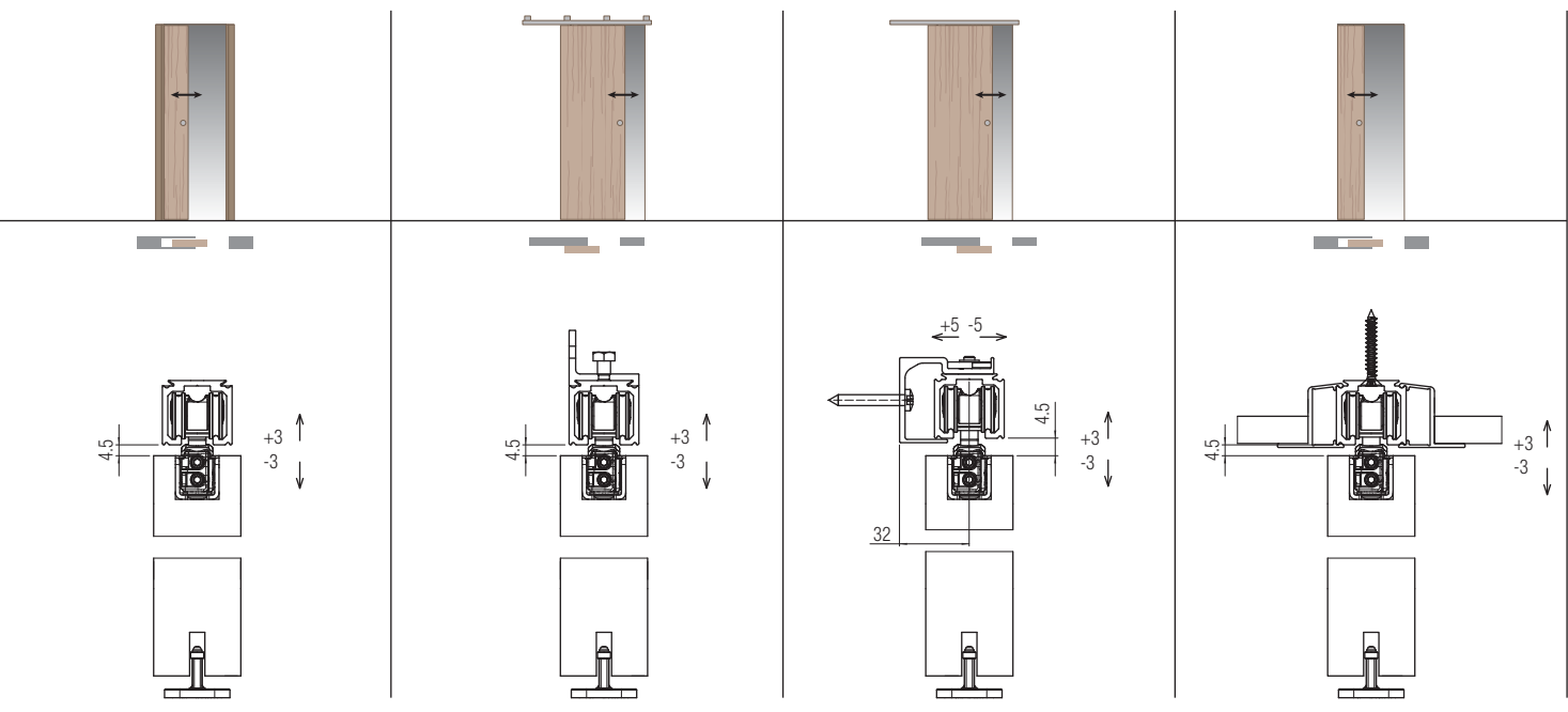
ABS + ABS Арт. 0600/50 2ABS
