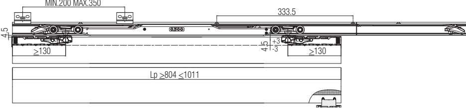
ABS + STOPPER Арт. 0600/80 1ABS
