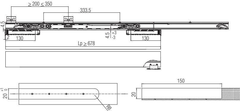
ABS + STOPPER Арт. 0600/50 1ABS
