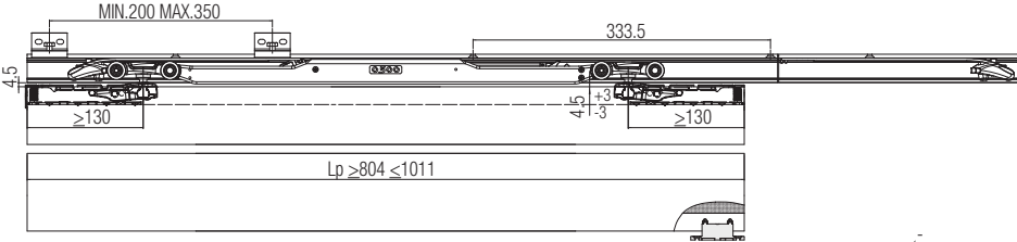
ABS + STOPPER Арт. 0600/50 1ABS
